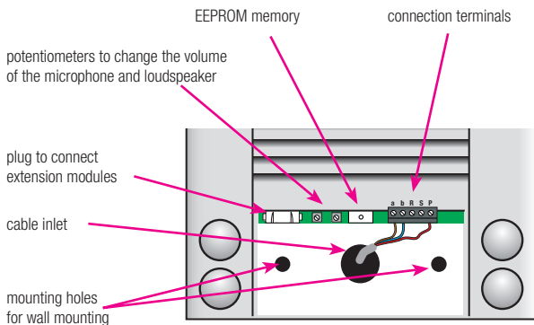
Fig. 2: making connection terminals and mounting holes visible
