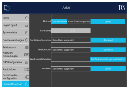
Abb. 19: Menü Upload/Download
