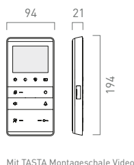
Video-2-Draht TASTA Video
